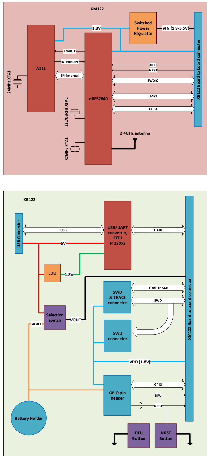
Figure 1 The block diagram of the EVK.
