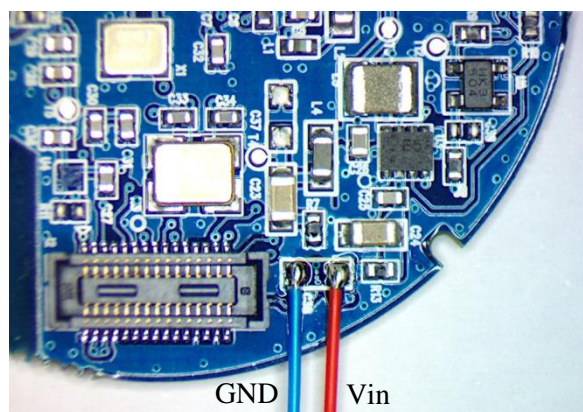
Figure 2: Connecting external power to the XM122.
